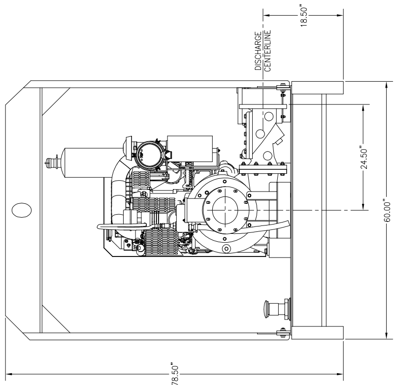
END VIEW
